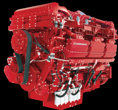
QSX78 2750 kWe
